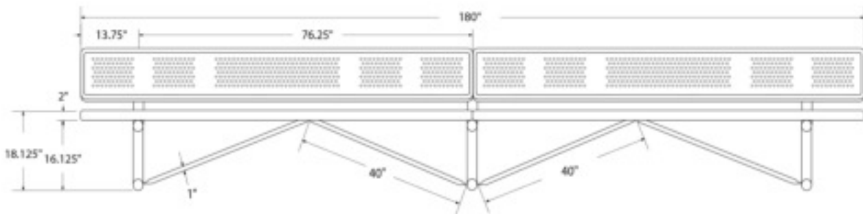
side view
