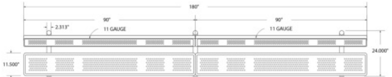
top view
